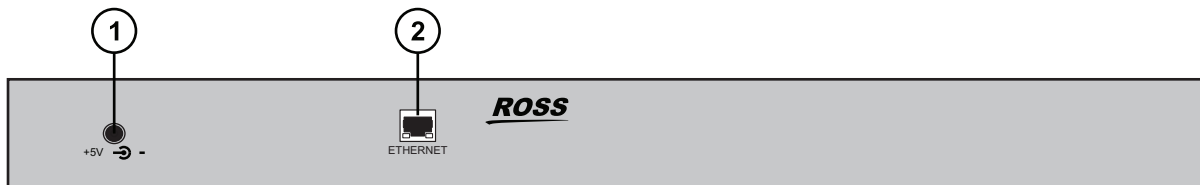
Figure 6 Rear Panel of an RCP-ME
